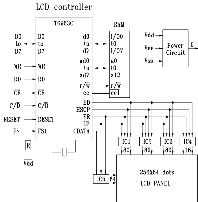
Block diagram
